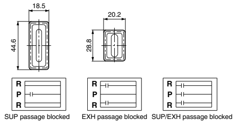
SUP passage blocked EXH passage blocked SUP/EXH passage blocked
