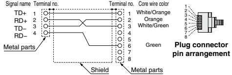
Connections (Straight cable)
