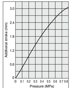
Additional Stroke due to Pressure on Each Side (MY3A32)
