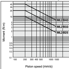
ML2B/M 1 (Pitch moment)
