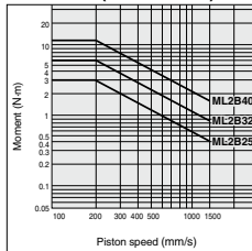
ML2B/M 3 (Yaw moment)
