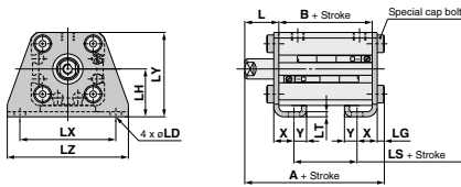
Male rod end
