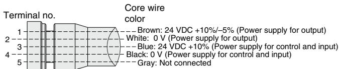
Connections (PROFINET)
