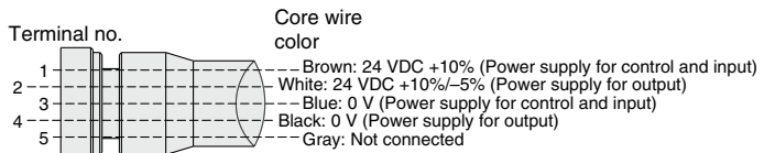
Connections (EtherNet/IP™)
