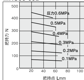
MHSJ3-63D
