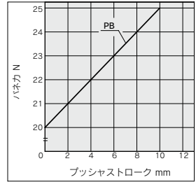
MHSH3-63DB
