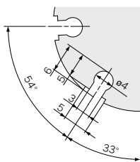
MHS3-20D
