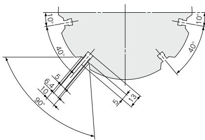
MHS3-100D
