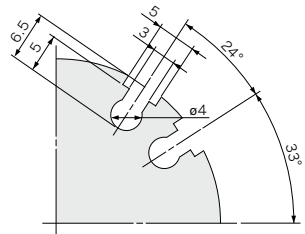
MHS2-25D
