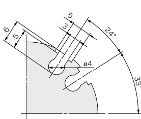
MHS2-20D
